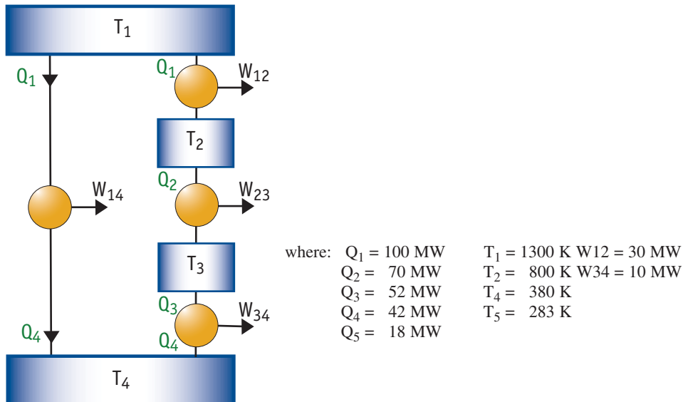
Figure A7.5 – Identical real heat engines
