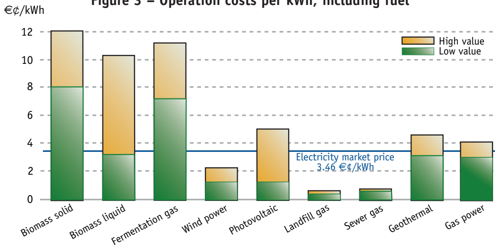
Figure 3 – Operation costs per kWh, including fuel
