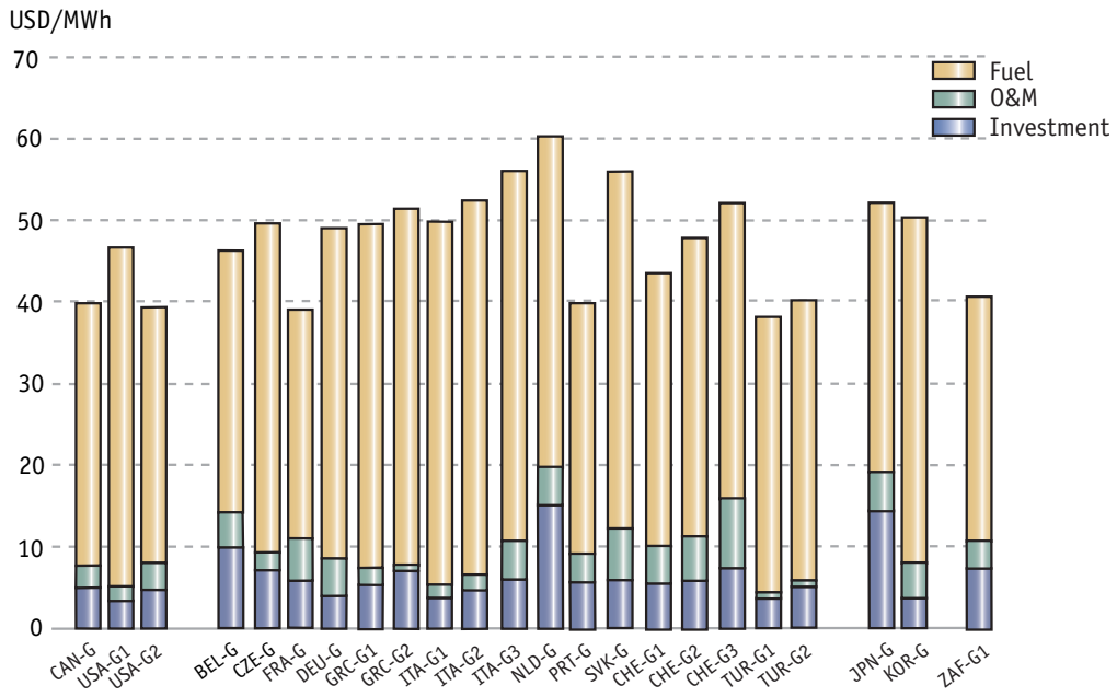
Figure 3.5 – Levelised costs of gas generated electricity at 5% discount rate (USD/MWh)
