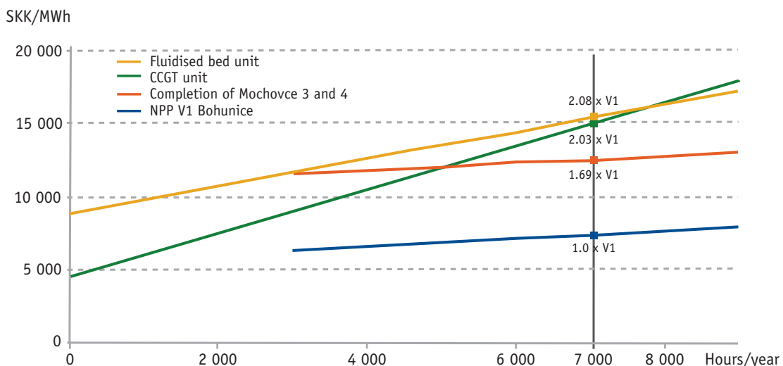
Figure 1a – Generation costs at different NPP annual hours of plant utilisation (not including external costs)
