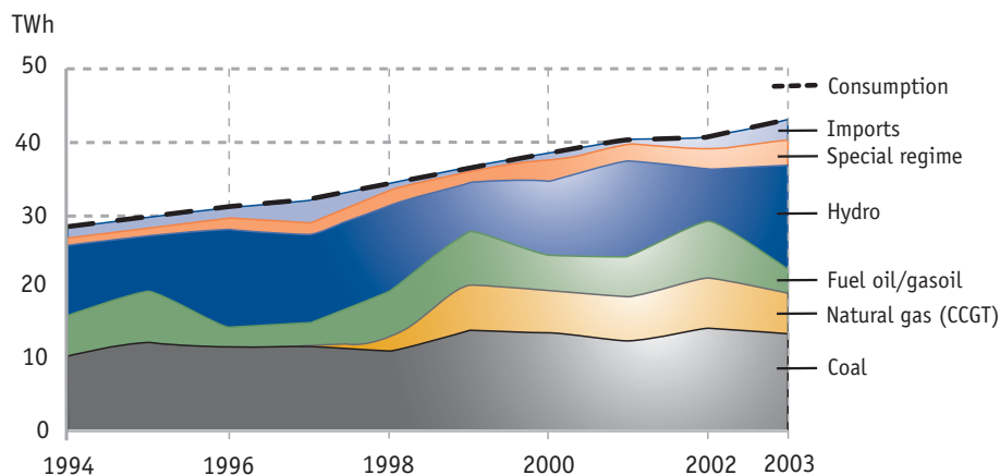
Figure 1 – Generation and consumption evolution
