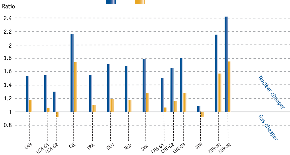
Figure 3.13 – Cost ratios for gas-fired and nuclear power plants at 5% and 10% discount rates
